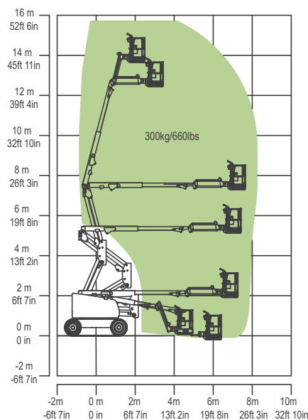
Range of Motion ZA14J (ZA45J)
